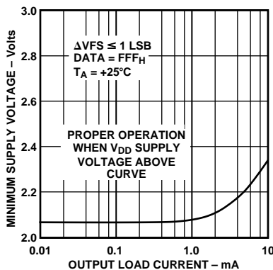
Figure 1. Minimum Supply Voltage vs. Load
